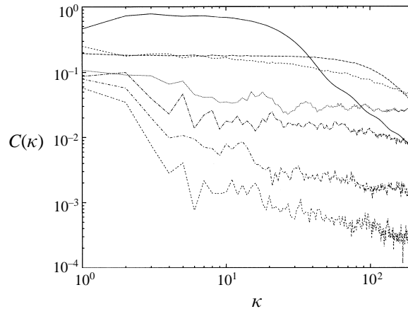
FIGURE 22. C(\kappa) vs. \kappa for n = 1 to 64 for \varepsilon = 0.1 , k = 1 , c = 3 and \delta_c = 0.2 , \tau = 0.5T . n increases by powers of two as one goes downwards. The initial distribution consists of 63 886 points inside f(L_{2,1}(1)) (for \varepsilon = 0.1 and \delta_c = 0 ) and 40 000 divisions are used; other details of the calculation are as in figure 10. Note the shallowness of the spectra.
